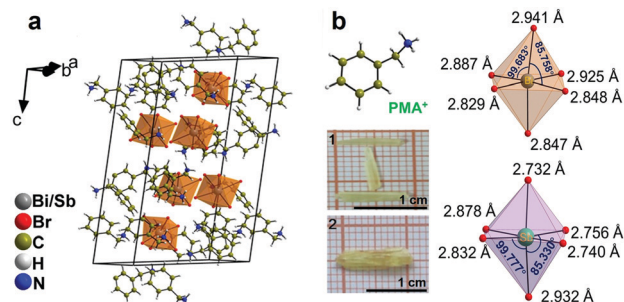
Fig. 1 (a) Crystal structures of 1 and 2 . (b) Structure of the organic cation of PMA + , photographs of single crystals of 1 and 2 , and distorted octahedra in 1 and 2 , respectively.
