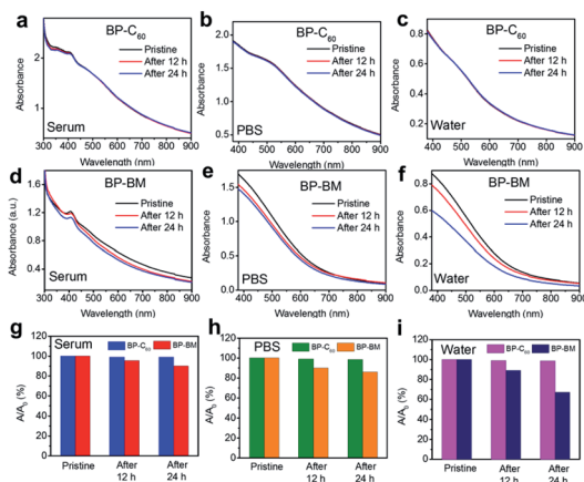
Fig. 2 Stability of the BP-C 60 hybrid and BP-BM dispersions in serum, PBS and water. UV vis absorption spectra of the BP-C 60 hybrid (a–c) and BP-BM (d–f) dispersed in serum (a and d), PBS (b and e) and water (c and f) after standing for 12 and 24 hours. Variation of the absorption ratios ( A/A_0 ) at 460 nm of the BP-C 60 hybrid and BP-BM dispersed in serum (g), PBS (h) and water (i) after standing for 12 and 24 hours.
