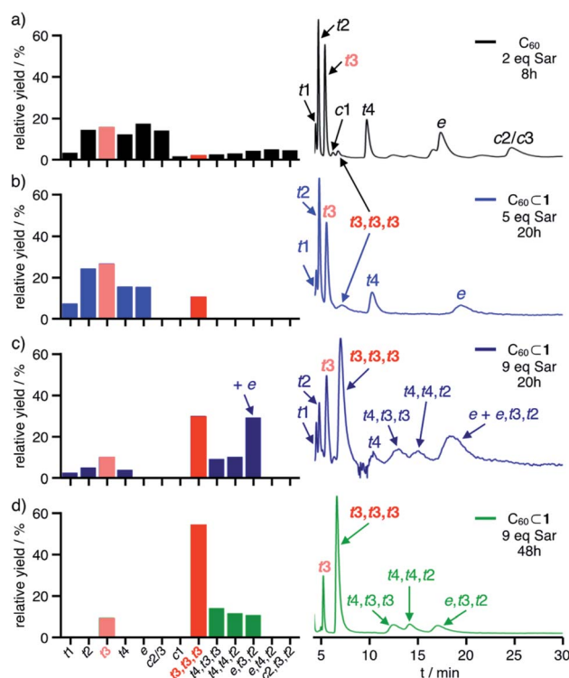
Fig. 5 Relative yields (left, calculated from HPLC profiles) for bisadducts 3 and trisadducts 4 and HPLC chromatograms (right) for (a) control experiment with C_{60} (2.0 eq. Sar, 8 h) and cage-templated reactions with C_{60}\subset 1 and (b) 5 eq. Sar (20 h), (c) 9 eq. Sar (20 h) and (d) 9 eq. Sar (48 h, preparative scale); yields for 3- t3 and 4- t3,t3,t3 are indicated in light red and red, respectively.
