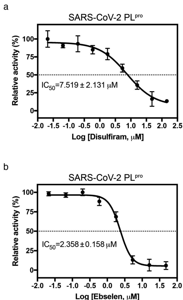
Fig. 3 Inhibition of SARS-CoV-2 PL pro by disulfiram and ebselen. The protease activity of PL pro ( 0.5 \mu\text{M} ) in the presence of 0 – 144 \mu\text{M} disulfiram (a) or 0 – 48 \mu\text{M} ebselen (b) was assayed using a fluorogenic substrate ( 50 \mu\text{M} , Dabcy-FTLKGGAPTKVTE-Edans-NH 2 ). The IC 50 value was determined by sigmoidal nonlinear regression logistic four parameter analyses using GraphPad Prism software ( n = 3 , error bars denote standard deviation).
