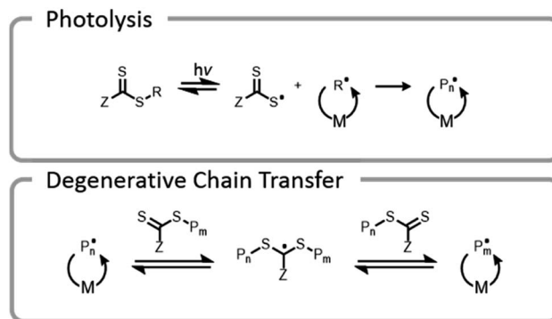
Fig. 9 Photoiniferter RAFT mechanism; M denotes monomer and P n denotes growing polymer chain; the CTA can undergo homolytic bond cleavage and the R group can initiate polymer chains. The growing chains can either recombine with the radical thio-carbonylthio-Z group (reversible deactivation) or undergo degenerative chain transfer.
