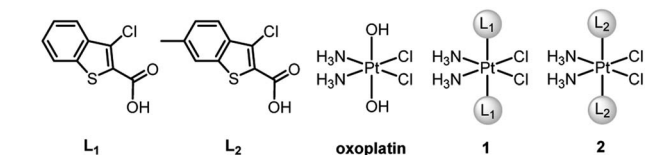
Fig. 1 Chemical structures of ligands L 1 and L 2 , oxoplatin and complexes 1 and 2 .
