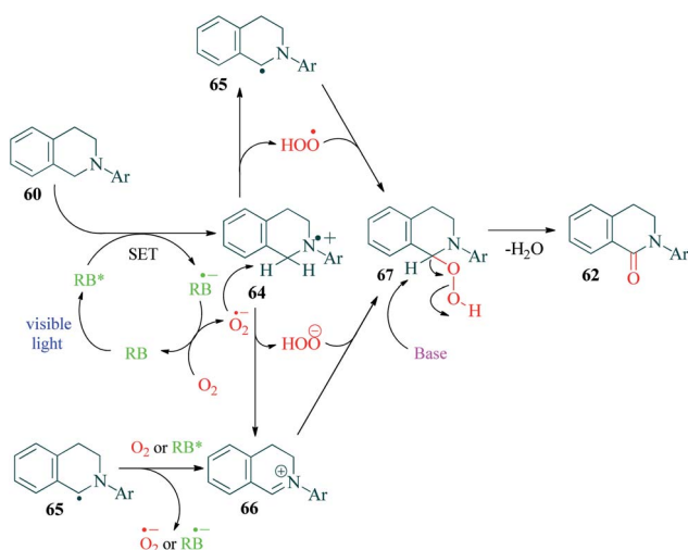
Scheme 18 Rose Bengal catalyzed C–H oxidation of tryptoline and tetrahydroquinoline substrates.
