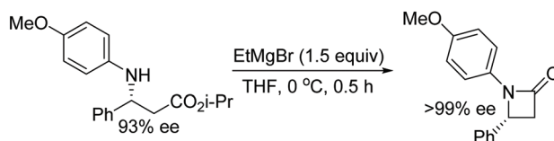
Fig. 58 CPA catalysed ATH of β-N-substituted enamino esters and construction of chiral β-lactam.
