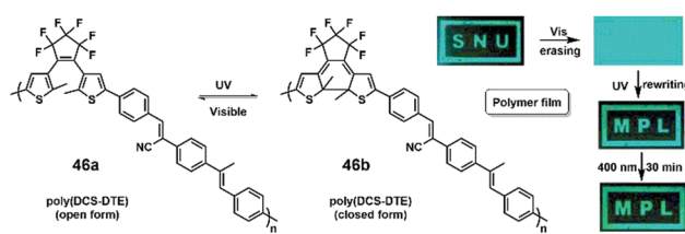
Fig. 20 Photochromic reactions of polymer 46a and erasable fluorescence imaging on a spin-coated polymer 46a film. Reproduced with permission. 59 Copyright 2005, American Chemical Society.
