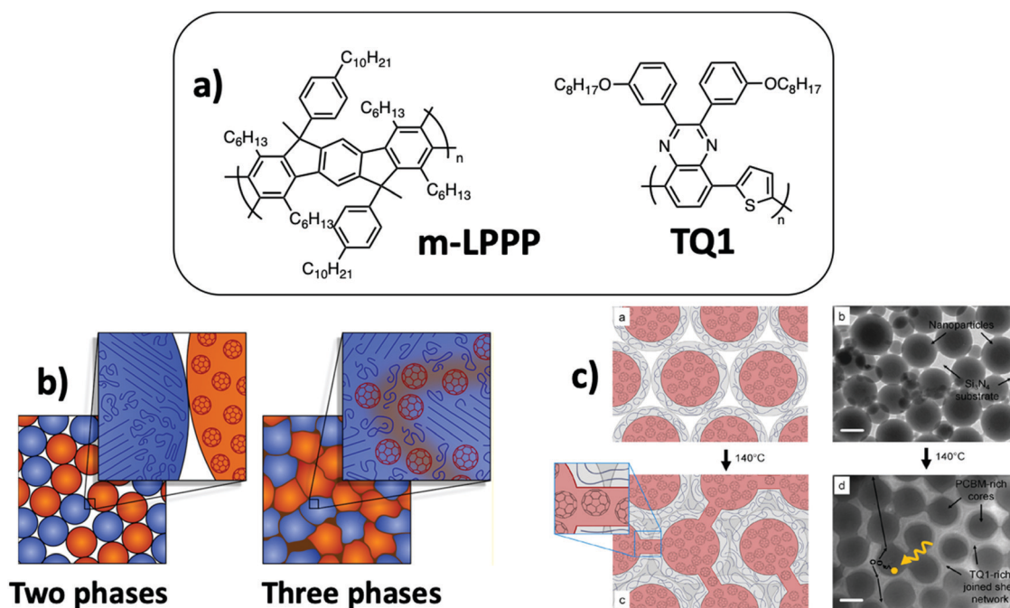
Fig. 13 (a) m-LPPP and TQ1 chemical structures. (b) Schematic representation of the three phase film microstructure obtained by thermal annealing of the assembly of PCBM NPs and P3HT NPs comprising crystalline P3HT and amorphous P3HT subdomains. A third mixed phase is obtained by sintering and diffusion of PCBM in the P3HT amorphous domains. Adapted with permission from ref. 71 (Copyright 2018 American Chemical Society). (c) Schematic representation and TEM images of composite NPs made of a PCBM -rich core and an amorphous TQ1 -rich shell. The mobility of the TQ1 polymer chains during thermal annealing slightly above its T_g allowed the movement of PCBM molecules and creation of bridging pathways between the PCBM -rich cores. Adapted with permission from ref. 74 (Copyright 2016 Elsevier B.V.).
