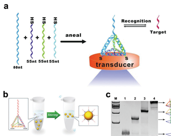
Fig. 3 DNA tetrahedra assembled by thiolated DNA strands (a) or carboxyl group modified DNA strands (b). (c) Analysis of DNA tetrahedra by PAGE. Figures reproduced with permission from: a, ref. 58. Copyright 2010, Wiley-VCH; b and c, ref. 59. Copyright 2015, American Chemical Society.
