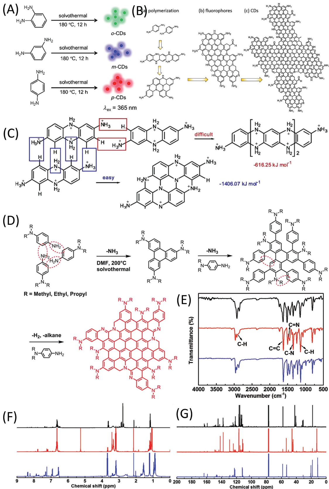
Fig. 8 (A) Preparation of RGB PL CDs from three different phenylenediamine isomers (o-PDA, m-PDA, and p-PDA). 62 (B) Illustration of the formation process of CDs based on the polymerization of PPD. (a) Polymerization of PPD, (b) formation of nitrogen-containing fluorophores, and (c) possible structure of CDs. 64 (C) Formation energies of longitudinal and transverse growths of a dimer of p-PDA. 67 (D) Synthesis of CD-NMe 2 , -NEt 2 , and -NPr 2 via solvothermal treatment of N,N-dimethyl-, N,N-diethyl-, and N,N-dipropyl-p-PD, respectively. (E) FTIR, (F) 1 H NMR, and (G) 13 C NMR spectra of CD-NMe 2 (black), -NEt 2 (red), and -NPr 2 (blue). 68
