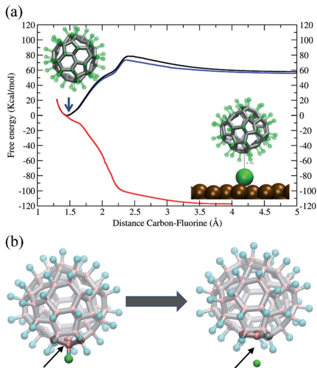
Fig. 6 (a) Free energy profile (potential of mean force) for moving a selected F atom away from C 60 F 48 as a function of the C–F separation. In absence of any surface (black line), in the presence of a Ni(111) surface at a \sim 7 Å of the C atom of the closest C–F bond (blue line) and at a distance of \sim 5.45 Å between the C atom of the C–F bond and the Ni(111) surface (red line). The two snapshots within the plot illustrate the equilibrium state (black arrow) and the final state with the F atom adsorbed at an arbitrary location of the Ni(111) surface, respectively. (b) Snapshots before and after extraction of an F atom from C 60 F 48 during the free energy calculations in (a). Note the structural change of the molecular cage. Left: C 60 F 48 structure equilibrated at 300 K, the C–F bond considered is indicated (arrow). Right: structure equilibrated at 300 K with an F atom maintained at a distance of 2.75 Å from the nearest C atom (larger than the sum of covalent radius but smaller than the sum of van der Waals radius).
