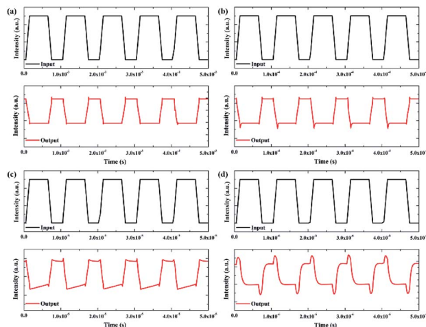
Fig. 6 Temporal response characteristics of an NVCT-based inverter with various square wave input signals of (a) 100 \mu\text{s} , (b) 10 \mu\text{s} , (c) 100 ns and (d) 10 ns.
