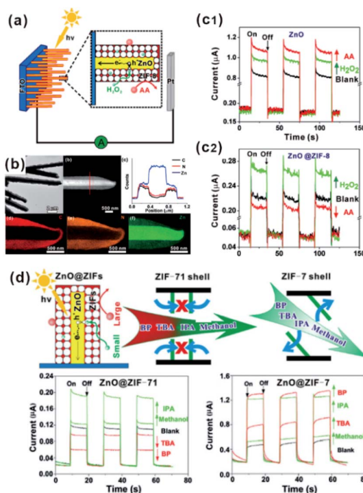
Fig. 10 (a) Schematic illustration of the PEC sensor with good selectivity towards H 2 O 2 . (b) Low-magnification TEM image, HAADF-STEM image, cross-sectional compositional line profiles and elemental maps of ZnO@ZIF-8 nanorods. (c1 and c2) Photocurrent response of ZnO and ZnO@ZIF-8 nanorod arrays. Reproduced with permission. 26 Copyright©2013 American Chemistry Society. (d) Schematic illustration of the ZnO@ZIF based PEC sensor (ZnO@ZIF-7 vs. ZnO@ZIF-71) with molecular size selectivity. Reproduced with permission. 60 Copyright©2016 The Royal Society of Chemistry.
