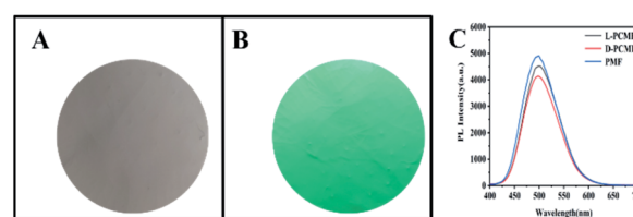
Fig. 2 Digital photos of the L -PCMF fluorescent polymer nanofiber membrane: (A) the membrane under sunlight; (B) the membrane under UV light of 365 nm; (C) fluorescence emission spectra of the three fluorescent polymer membranes (365 nm excitation).
