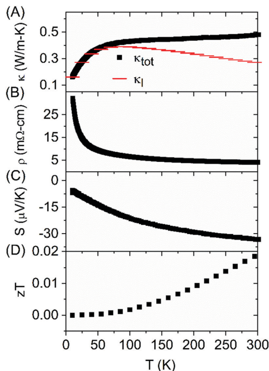
Fig. 5 Total thermal conductivity ( \kappa_{\text{tot}} ) and lattice thermal conductivity ( \kappa_{\text{l}} ) (A), resistivity (B), Seebeck coefficient (C), and zT (D) measured on a \text{FeAs}_{1.50}\text{Se}_{0.50} single crystal.
