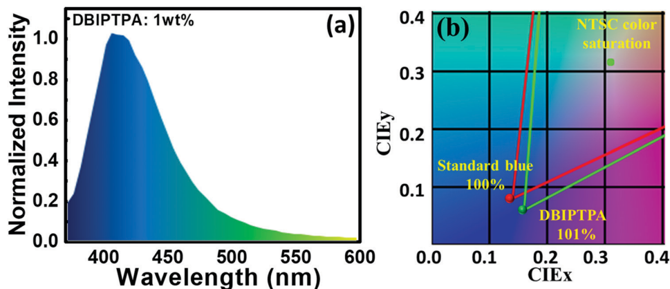
Fig. 12 (a and b) EL spectrum and NTSC color saturation of the solution-processed OLEDs containing 1 wt% DBIPTPA as the emitter at the brightness of 100 cd m -2 , respectively.
