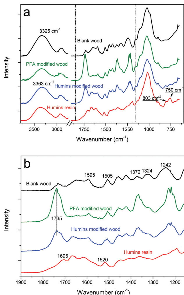
Fig. 1 (a) IR spectra of blank wood (black line), PFA modified wood (green line), humin modified wood (blue line) and humin resins (red line) (a) in the range 3800 \text{cm}^{-1} –700 \text{cm}^{-1} and (b) zoom on the region 1900 \text{cm}^{-1} –1100 \text{cm}^{-1} .
