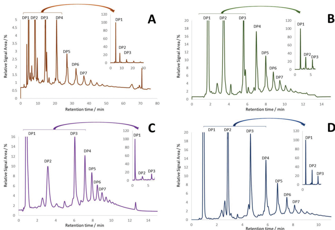
Fig. 2 HPLC-FLD chromatograms of the cocoa extract calibrant using different HPLC columns: (A) Nomura Develosil Polar Diol 4.6 × 250 mm, 5.0 μm particle size, 120 Å pore size; (B) Phenomenex Luna Diol 4.6 × 100 mm, 3.0 μm particle size, 200 Å pore size; (C) Supelco Kromasil Diol 2.1 × 100 mm, 5.0 μm particle size, 100 Å pore size and; (D) Waters Torus Diol 3.0 × 100 mm, 1.7 μm particle size, 130 Å pore size.
