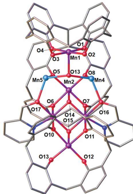
Fig. 3 Side (A) and orthogonal (B) views of the partial single crystal X-ray structure of the asymmetric unit in 6 . Selected labels have been added according to discussion. Colour code C – grey, O – red, N – royal blue, Mn II – pale blue, Mn III – purple. Hydrogen atoms, t Bu groups, ligated solvent molecules and co-crystallised solvent/anions omitted for clarity. Figures not to scale.
