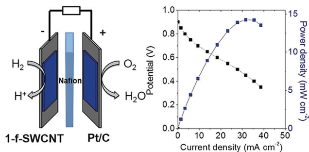
Fig. 11 Polarization (black) and power density (blue) curves for an MEA employing [\text{Ni}(\text{P}_2^-\text{N}_2^{\text{Arg}})_2]^{7+} (denoted as 1-f-SWCNT) and Pt/C as the anode and cathode catalysts, respectively. Experimental conditions: anode loading: 0.3 \mu\text{g cm}^{-2} , cathode loading (Pt/C): 1 \text{ mg cm}^{-2} , Nafion ® as the polymer electrolyte, 60 \text{ }^\circ\text{C} cell temperature. Reprinted with permission from ref. 297. Copyright 2017 Wiley-VCH.
