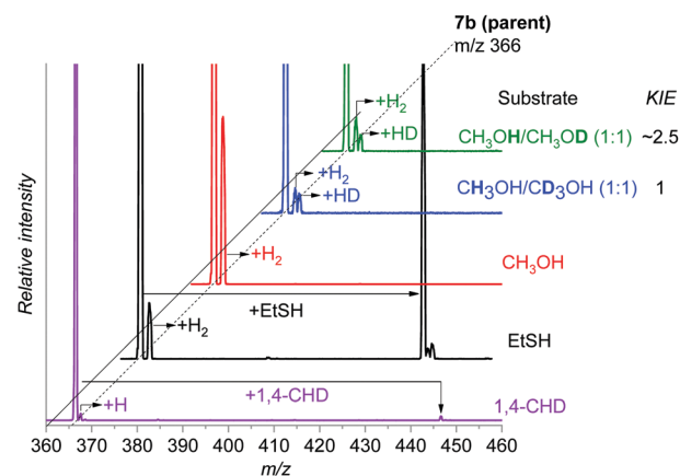
Fig. 4 Gas phase reactivity of 7b with 1,4-cyclohexadiene (purple), ethanol (black), methanol (red), CH 3 OH/CD 3 OH (1:1) (blue), and CH 3 OH/CH 3 OD (1:1) (green). The experiments were performed at zero collision energy with a pressure of the reactant gas of 0.2 mTorr, except for 1,4-cyclohexadiene for which it was raised to 0.3 mTorr (see also Fig. S11, ESI†). The relative concentrations of the isotopically labelled methanols were determined by an association reaction with the [Au(PMe 3 )] + cation (see the ESI† for details).
