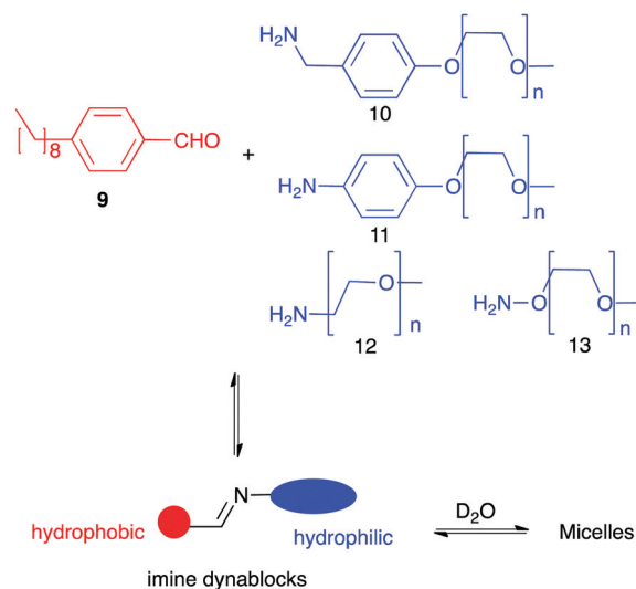
Fig. 6 Formation of supramolecular aggregates using Imine dynamlocks reported by Giuseppone. 55
