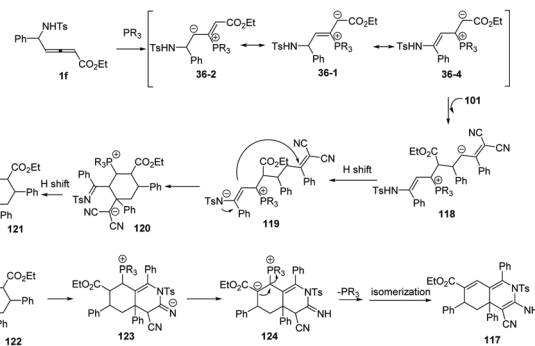
Scheme 38 Proposed mechanism.
