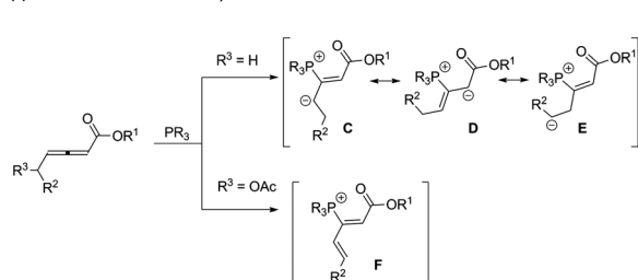
Scheme 1 The reactivity of allenates in the presence of organophosphines.
