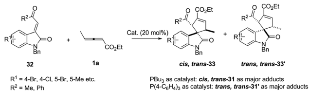
Scheme 9 Phosphine-catalysed stereoselective dearomatization of 3- \text{NO}_2 -indoles.
