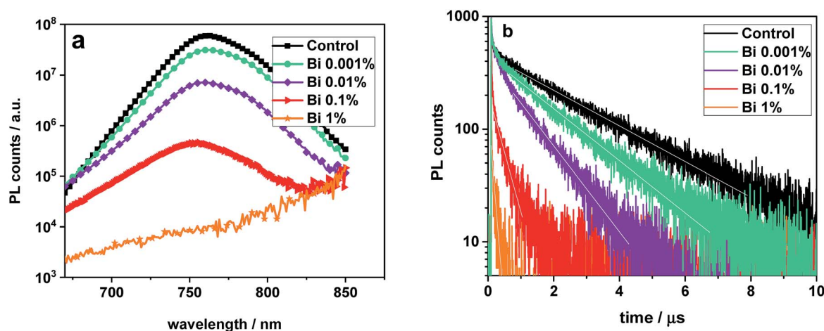
Fig. 4 Photoluminescence of perovskite films (a) absolute PL spectra showing that adding Bi reduces the PL yield so substantially that it is hardly detectable for [\text{Bi}] = 1\% . (b) Transient PL with a reduced decay time for higher Bi concentrations. The white lines are mono-exponential fits and span the time range selected for the fits.
