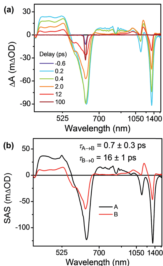
Fig. 8 (a) fsTA spectra and (b) species-associated spectra (SAS) of Per ⊂ TTzExVBox 3++ in CH 3 CN excited at 620 nm ((A) 2 *TTz 2+ (D n ), (B) TTz 2+ -Per-ExV + ). The wavelength axis is plotted in reciprocal space. Time constants are for the representative data set shown here; averages and standard deviations from multiple experiments are given in Table 1.
