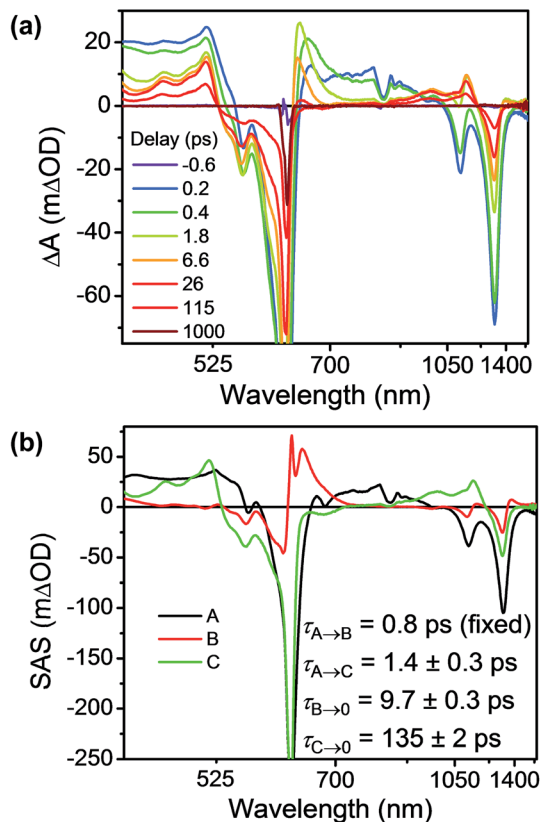
Fig. 7 (a) fsTA spectra and (b) species-associated spectra (SAS) of TTzExVBox 3++ in CH 3 CN excited at 620 nm ((A) 2 *TTz 2+ (D n ), (B) 2 *TTz 2+ (D 1 ), (C) TTz 2+ -ExV + ). The wavelength axis is plotted in reciprocal space. Time constants are for the representative data set shown here; averages and standard deviations from multiple experiments are given in Table 1.
