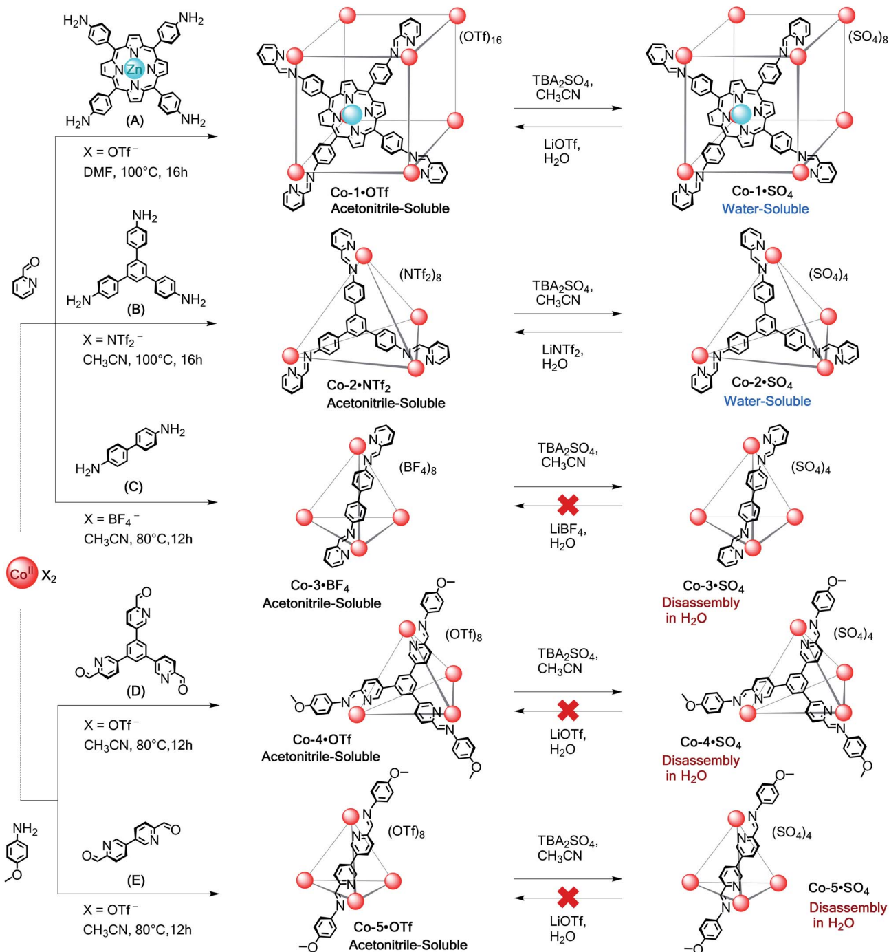
Scheme 1 Subcomponent self-assembly of \text{Co}^{\text{II}} -capsules. Preparation of acetonitrile-soluble Co-1 · \text{X} to Co-5 · \text{X} ( \text{X} = \text{OTf}^- , \text{NTf}_2^- , or \text{BF}_4^- ) from subcomponents A – E and their anion exchange sequences.
