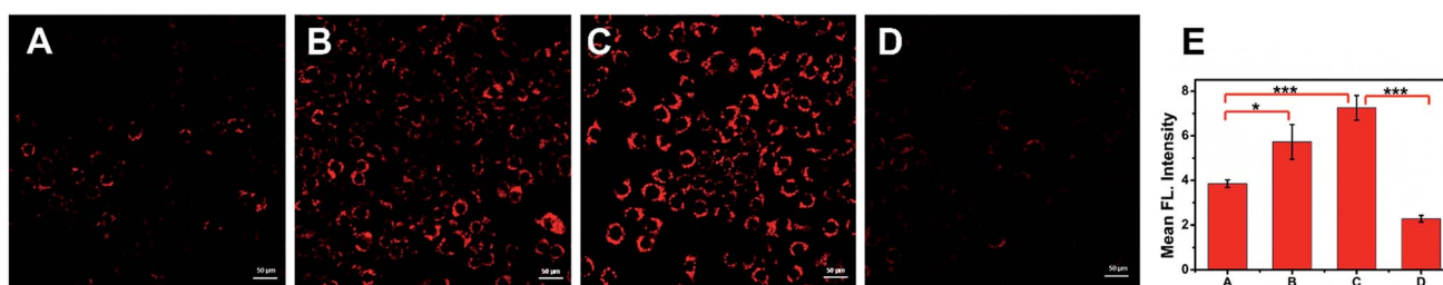
Fig. 2 Laser confocal imaging of O_3 in RAW 264.7 macrophages. (A) Cells incubated with 10 \mu M ACy7 for 15 min at 37 °C. (B) ACy7-loaded cells incubated with 5 \mu M O_3 for 10 min. (C) Cells incubated with PMA (100 ng mL −1 ) for 20 min and then incubated with 10 \mu M ACy7 at 37 °C for 15 min. (D) Cells incubated with PMA (100 ng mL −1 ) for 20 min, and then with 0.05 mM ethyl 4-vinylbenzoate for 30 min, and then with 10 \mu M ACy7 for 15 min. (E) The data output of the graphs in (A)–(D). All cells were washed 3 times with 0.01 M PBS prior to imaging. Emissions from 640 nm to 740 nm were collected using a 561 nm laser. The values are the mean \pm s.d. for n = 3 , * p < 0.05 , and *** p < 0.001 .
