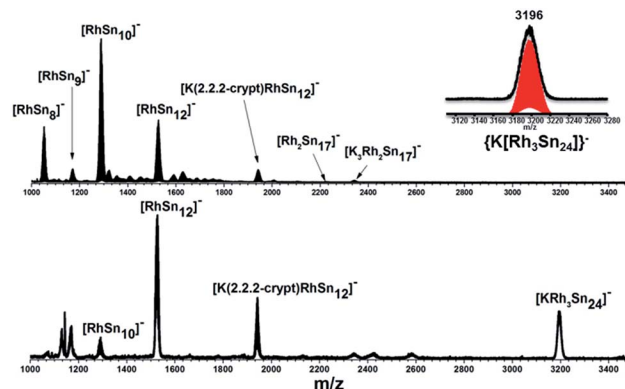
Fig. 1 ESI-MS ( m/z : 1000–3500) in negative ion mode of en(bottom) and DMF (up) reaction mixtures. The inset show the [\text{K}(\text{Rh}_3\text{Sn}_{24})]^- peak and its simulated pattern.
