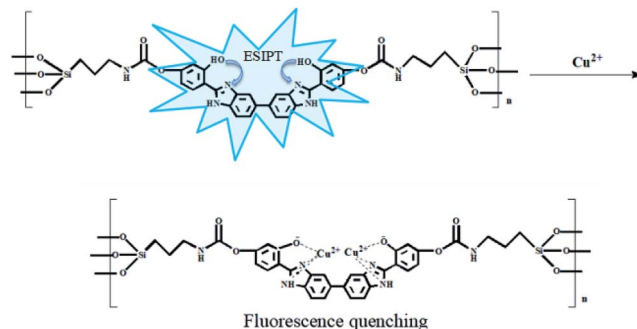
Fig. 9 The mechanism of BBM-PMO detection of Cu 2+ .
