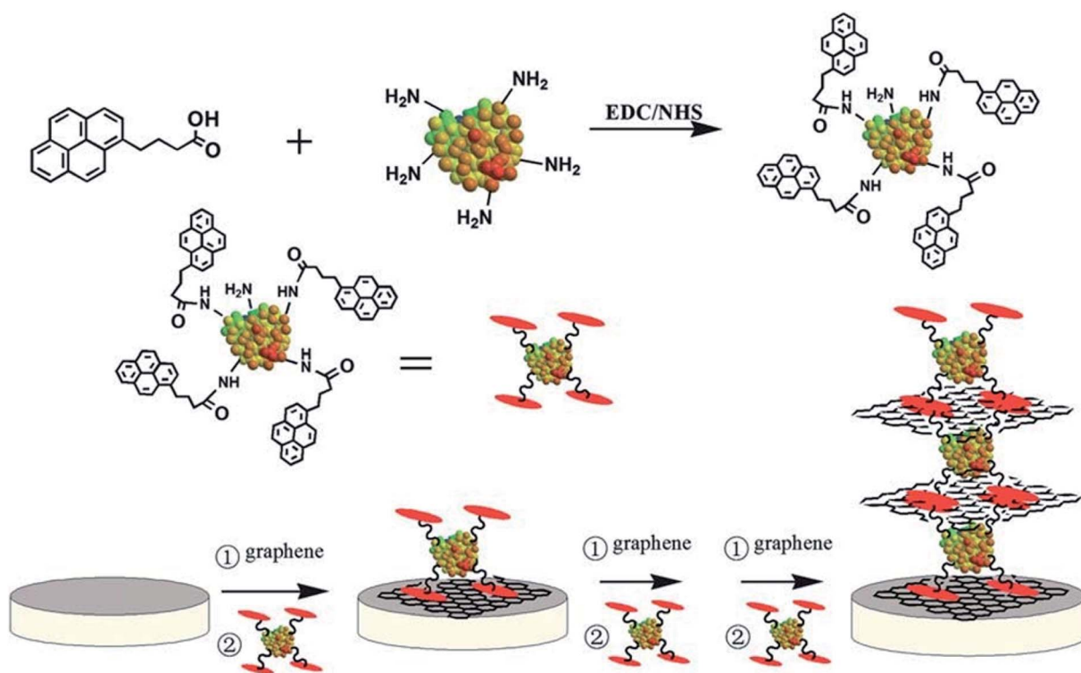
Fig. 5 Schematic illustration of the immobilization of GOx enzymes on graphene via pyrene and the subsequent fabrication of single- and multi-layered enzyme electrodes. [Reprinted with permission from ref. 196, J. Liu, N. Kong, A. Li, X. Luo, L. Cui, R. Wang and S. Feng, Graphene Bridged Enzyme Electrodes for Glucose Biosensing Application, Analyst , 2013, 138 , 2567–2575. Copyright© Royal Society of Chemistry.]
