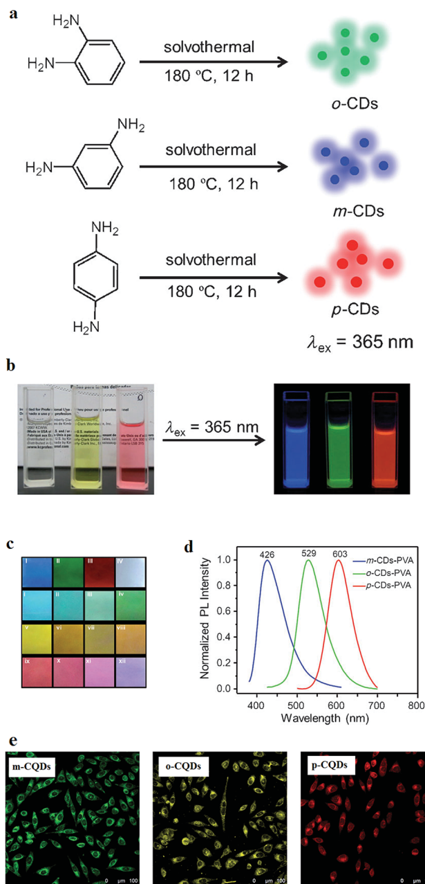
Fig. 5 (a) Synthesis method of CQDs from phenylenediamine isomers, oPD, mPD and pPD that results in o-CQDs, m-CQDs, and p-CQDs, respectively. (b) Photographs of the ethanol solutions of o-CQDs, m-CQDs, and p-CQDs in daylight (left) and under UV excitation with the wavelength of \lambda = 365 \text{ nm} (right), (c) the m-CQDs, o-CQDs, p-CQDs mixtures in PVA films under excitation with a wavelength of \lambda = 365 \text{ nm} : (I) m-CQDs; (II) o-CQDs; (III) p-CQDs; (IV) o-CQDs/m-CQDs/p-CQDs = 2 : 4 : 1 (w/w/w); (i–iv) o-CQDs/m-CQDs = 1 : 8, 1 : 4, 1 : 2, and 1 : 1; (v–viii) o-CQDs/p-CQDs = 4 : 1, 2 : 1, 1 : 1, and 1 : 2; (ix–xii) m-CQDs/p-CQDs = 1 : 4, 1 : 2, 1 : 1, and 4 : 1 (all ratios are w/w), (d) the normalized PL spectra of the PVA films with m-CQDs, o-CQDs, and p-CQDs (UV excitation of \lambda = 365 \text{ nm} ), (e) confocal fluorescence microscopy of m-CQDs, o-CQDs and p-CQDs of MCF-7 cells at a constant laser excitation wavelength of 405 nm, reprinted with permission from ref. 154, copyright 2015 John Wiley and Sons.
