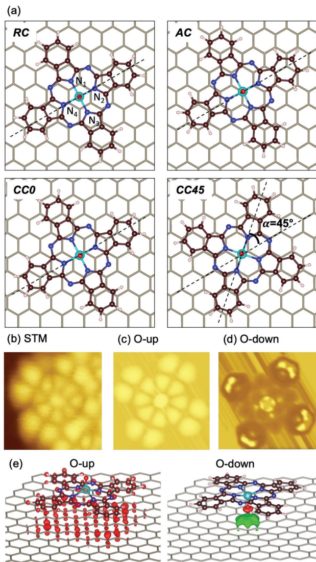
Fig. 3 (a) Configuration of VOPc on graphene considered for theoretical calculations. From top-left to bottom-right: ring-centered (RC), atom-centered (AC), C–C \alpha = 0^\circ (CC0) and CC/ \alpha = 45^\circ (CC45). Nitrogen atoms coordinated with vanadium atoms are numbered; the N_2VN_4 axis and the direction of graphene C–C bonds are indicated by dashed lines. (b) Experimental STM image of VOPc on Gr/SiC(0001) measured at V_b = 2 V (filled states); (c) simulated STM image of VOPc@Gr at a RC site having an O-up configuration and (d) O-down configuration ( V = -1.7 V, filled states). (e) Difference electronic density plots for O-up (left) and O-down (right) configurations.
