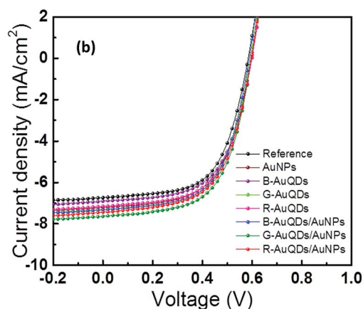
Fig. 2 (a) Schematic of the fabricated OSCs and (b) J - V characteristics of the OSCs compared with that of the reference cell.
