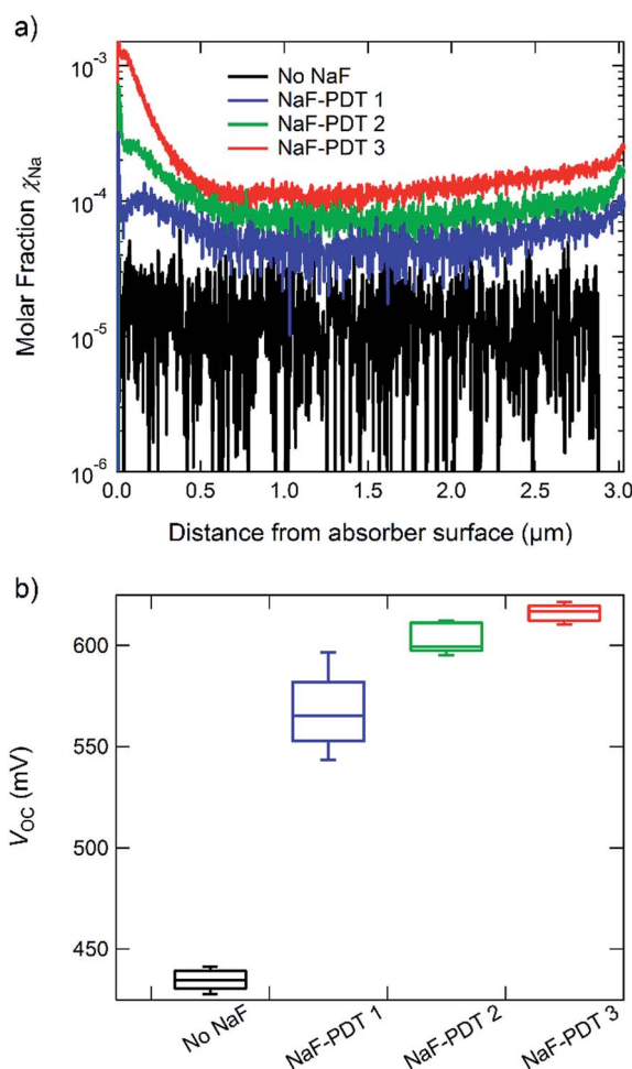
Fig. 5 (a) Molar fraction of Na of four different samples with different amounts of Na incorporated derived from GD-OES measurements. (b) Open-circuit voltage of the corresponding solar cells.
