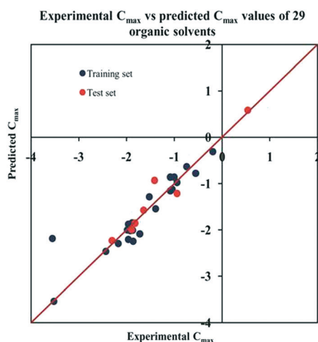
Fig. 12 The scatter plot of the observed and the predicted dispersibility index of SWCNTs ( \log C_{\max} ) of the developed PLS model (model P1).
