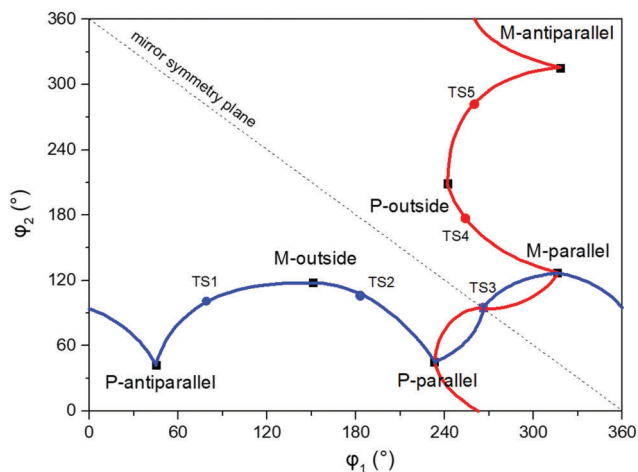
Fig. 3 Changes in the dihedral angles \varphi_1 and \varphi_2 during the reaction going from the P-antiparallel to the M-antiparallel form of DTE. Points on the red and blue curves on opposite sides of the line indicating mirror symmetry represent enantiomers. See Fig. 1 for a definition of the dihedral angles.
