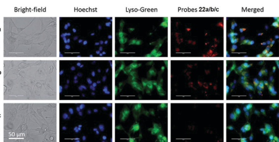
Fig. 32 Fluorescence images of MDA-MB-231 cells incubated with fluorescent probes 22a–c . Cells incubated with 5 \mu M of respective probes for 2 h, post serum starvation (2 h) and imaged for co-localization with 1 \mu M LysoSensor Green and (1 \mu g mL -1 ) Hoechst 33342 stains. All images were acquired at 60 \times magnification using an inverted fluorescence microscope (AMF-4306, EVOS FL , AMG). Copyright 2015 Royal Society of Chemistry.
