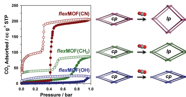
Fig. 3 \text{CO}_2 adsorption/desorption isotherms of flex MOF(CN), flex MOF(OH), and flex MOF( \text{CH}_2 ) at 196 K (left) and schematic of their flexible behaviours upon \text{CO}_2 adsorption (right). Filled and empty circles represent adsorption and desorption curves, respectively.
