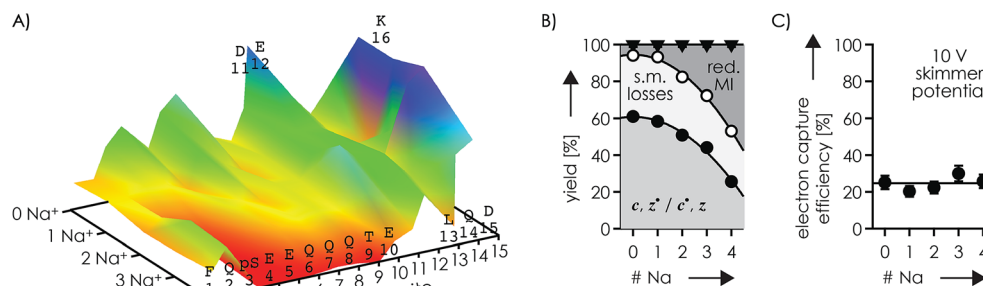
Fig. 3 (A) Site-specific fragmentation efficiency ( c , z^* and c^* , z fragments) from ECD of phosphopeptide ions with a net charge of 3+ and 0-4 \text{Na}^+ ions attached, with the color scale ranging from red (zero fragmentation) to yellow to green to blue (maximum fragmentation; detailed fragmentation efficiency values can be found in Fig. S7A and B†); (B) percentage stacked area plots illustrating the yield of c , z^* and c^* , z fragments, products from loss of small molecules (s.m.) from reduced molecular ions, and reduced molecular ions (including loss of \text{H}^+ ; loss of \text{Na}^+ was not observed) from ECD of phosphopeptide ions with a net charge of 3+ at 10 V skimmer potential, and (C) corresponding electron capture efficiency versus the number of \text{Na}^+ ions attached; solid lines in (B) are quadratic polynomial functions used for error analysis and that in (C) is meant to guide the eye.
