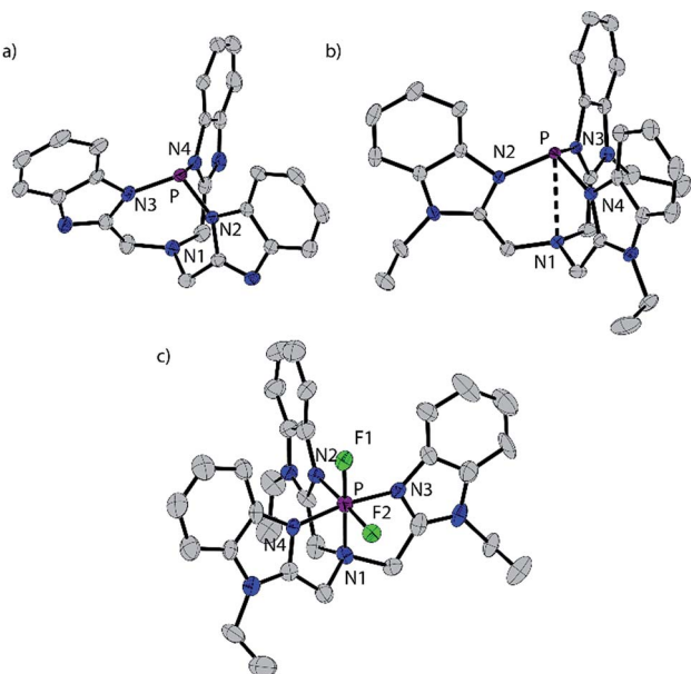
Fig. 1 Solid state structures of one of two independent molecules of P(BIM) (a), the cation in [\text{P}(\text{BIMe}_3)]^{3+}[\text{OTf}]_3 \cdot (\text{MeCN})_2 (b), and cation in [\text{PF}_2(\text{BIMe}_3)]^{3+}[\text{OTf}]_3 \cdot \text{MeCN} (c). Thermal ellipsoids are shown at a 50% probability level. Hydrogen atoms, solvent molecules and triflate anions are omitted for clarity. Inter-atomic distances and angles are summarized in Table 2.
