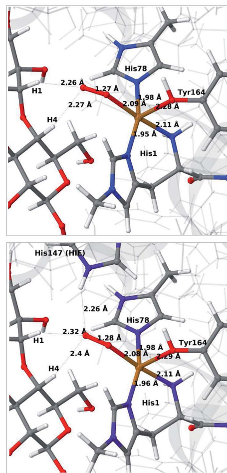
Fig. 3 QM/MM optimised [\text{CuO}_2]^+ ( 3 ) without (upper) and with (lower) His147 included in the QM region. Both optimisations were carried out with TPSS-D3/def2-SV(P) and system 2 fixed.
