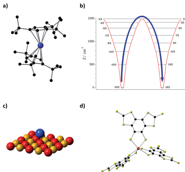
Fig. 5 (a) Molecular structure of [\text{Dy}(\text{Cp}^{\text{tnt}})_2]^+ , where \text{Cp}^{\text{tnt}} = \{\text{C}_5\text{H}_2^{\text{t}}\text{Bu}_3\text{-}1,2,4\} and ^{\text{t}}\text{Bu} = \text{C}(\text{CH}_3)_3 . H atoms are omitted for clarity. Dy: blue and C: black. (b) Energy levels and M_j projections of [\text{Dy}(\text{Cp}^{\text{tnt}})_2]^+ , determined by CASSCF-SO calculations. (c) Ho atom on a MgO monolayer. Mg: yellow and O: red. (d) Molecular structure of [\text{V}(\text{C}_8\text{S}_8)_3]^{2-} . V: red, C: black, and S: yellow.
