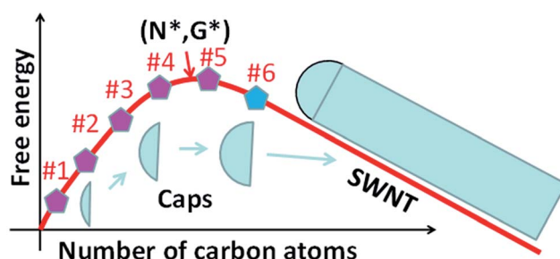
Fig. 3 The Gibbs free energy evolution during the nucleation and the growth of SWCNTs. The N* and G* denote the size of the nucleus and the nucleation barrier of the SWCNT. After the addition of the 6 th pentagon, N > N 6 , the cap becomes matured and the further elongation of the SWCNT thereafter results in a linear drop of the Gibbs free energy.
