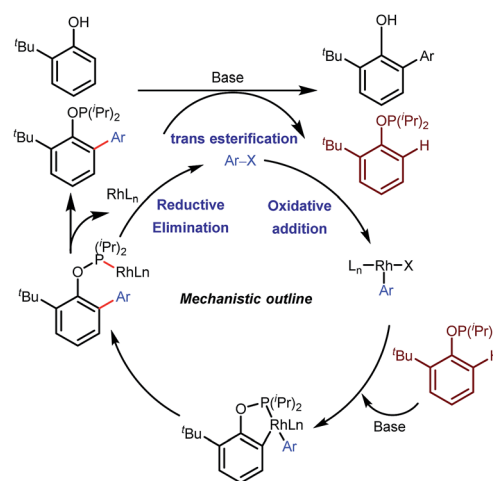
Fig. 6 Rh-catalyzed ortho -arylation of phenols using a phosphite tDG.
