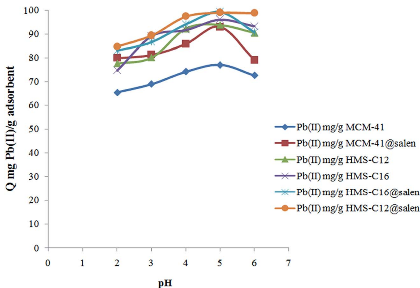
Fig. 9 Influence of pH solution on adsorption of Pb(II) (100 mg L -1 solutions) onto silicas.
