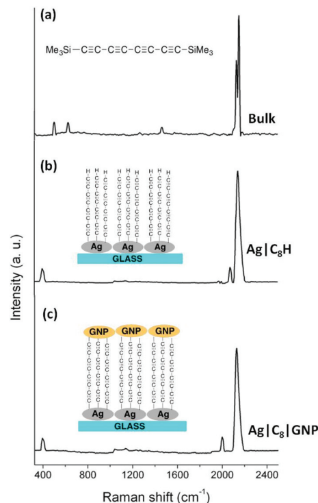
Fig. 2 (a) Raman spectrum of a powder sample of 1 ; (b) SERS spectrum of an \text{Ag|C}_8\text{H} film; and (c) SERS spectrum of an \text{Ag|C}_8|\text{GNP} film.
