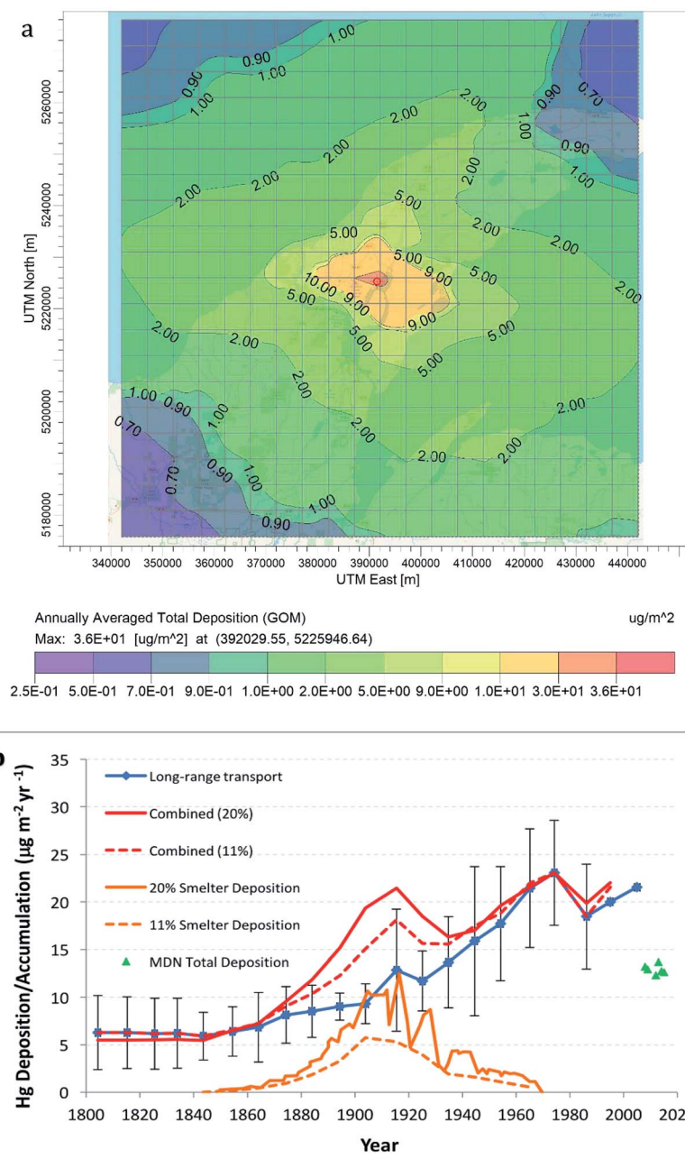
Fig. 7 Deposition of Hg from individual and collective smelters: (a) AERMOD modeling of Hg deposition around Calumet-Hecla Smelter. Shading shows relatively high deposition around smelter, yet distant dispersal around the Peninsula. (b) Smelter deposition from the 5 Keweenaw Waterway smelter emissions superimposed upon long-range deposition (Engstrom's values from 4 remote Wisconsin and Minnesota lakes 62,63 ). Green triangles show modern-day MDN total mercury deposition.
