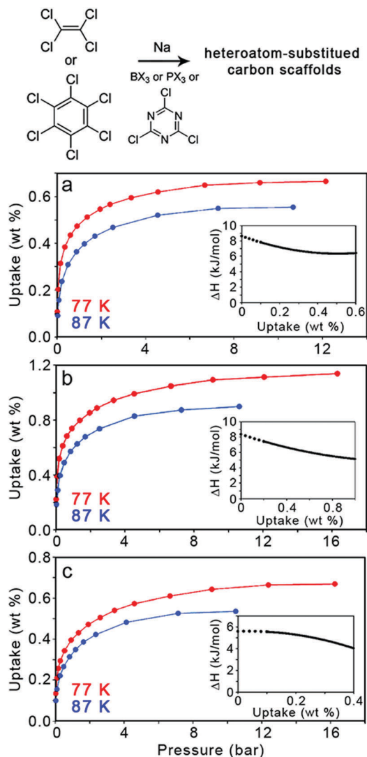
Fig. 14 (top) Bottom-up synthesis of heteroatom-substituted carbons; reaction conditions: tetraglyme, diphenyl ether, or paraffin oil solvent, X = halogen or OR, and temperatures between 250 and 350 °C. (bottom) Hydrogen uptake at 77 and 87 K for (a) boron-, (b) phosphorus-, and (c) nitrogen-substituted carbons. Adapted with permission from Z. Jin, Z. Z. Sun, L. J. Simpson, K. J. O'Neill, P. A. Parilla, Y. Li, N. P. Stadie, C. C. Ahn, C. Kittrell and J. M. Tour, J. Am. Chem. Soc. , 2010, 132 , 15246. Copyright 2008 American Chemical Society.
